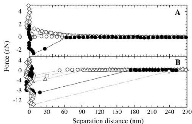
FIGURE 3 The forces between the functionalized silica particles and a freshly cleaved, mica plate in water of pH 5.6. Here, we used C1 - (□ with dotted line), C3 - (○ with dotted line), C6 - (△ with dotted line), C18 - (◇ with dotted line), and Plus -modified (● with solid line) silica particles. Panels A and B show the compression and decompression forces, respectively.
